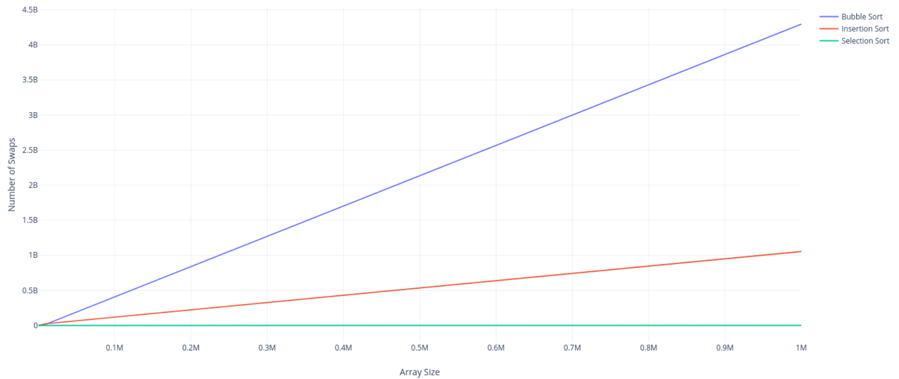
Number of Swaps (BS IS SS)
