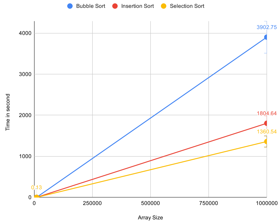
Time Complexities (BS IS SS)
